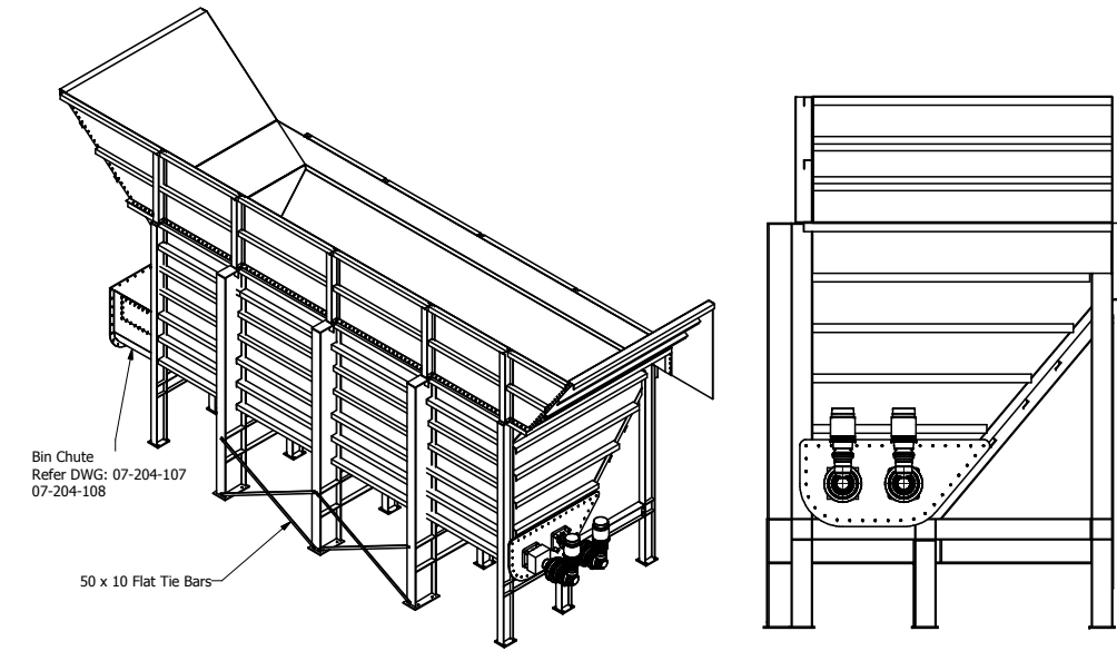
Left Elevation
