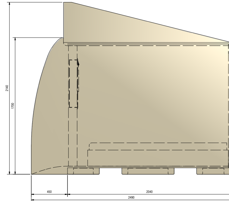
ELEVATION VIEW SCALE 1 / 10
